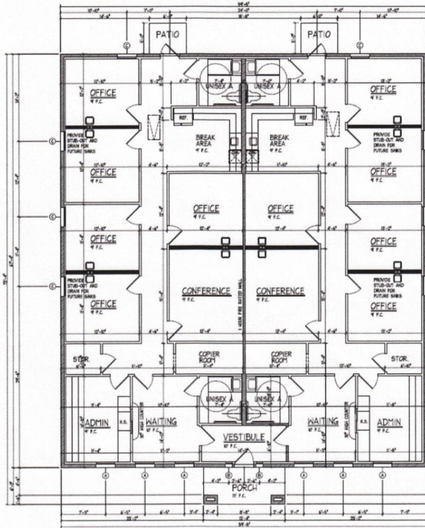
Floor Plan Building 1
